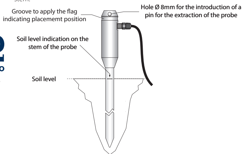
Fig. 2: installation
