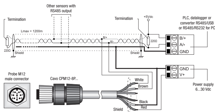
Fig. 4: RS485 connection
