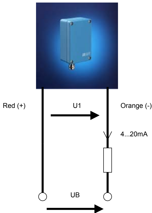
Illustration: Connection of the air pressure sensor
