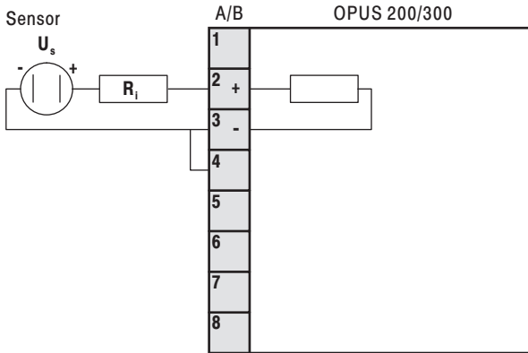
Figure 6: voltage measurement
