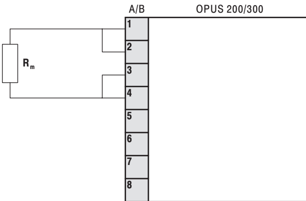
Figure 3: resistance measurement with 2-conductor technique
